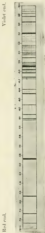
FIG. 31.—Spectrum of the electric gases.
